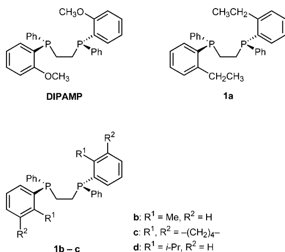
Figure 1. ( S,S )-DIPAMP and ( S,S )-bis[( o -alkylphenyl)phenylphosphino]ethanes.
