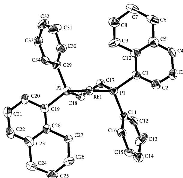
Figure 2. Molecular structure of cation complex 5c (ORTEP). Coordinated cyclooctadiene and counter anion ( \text{BF}_4^- ) are omitted for clarity.
