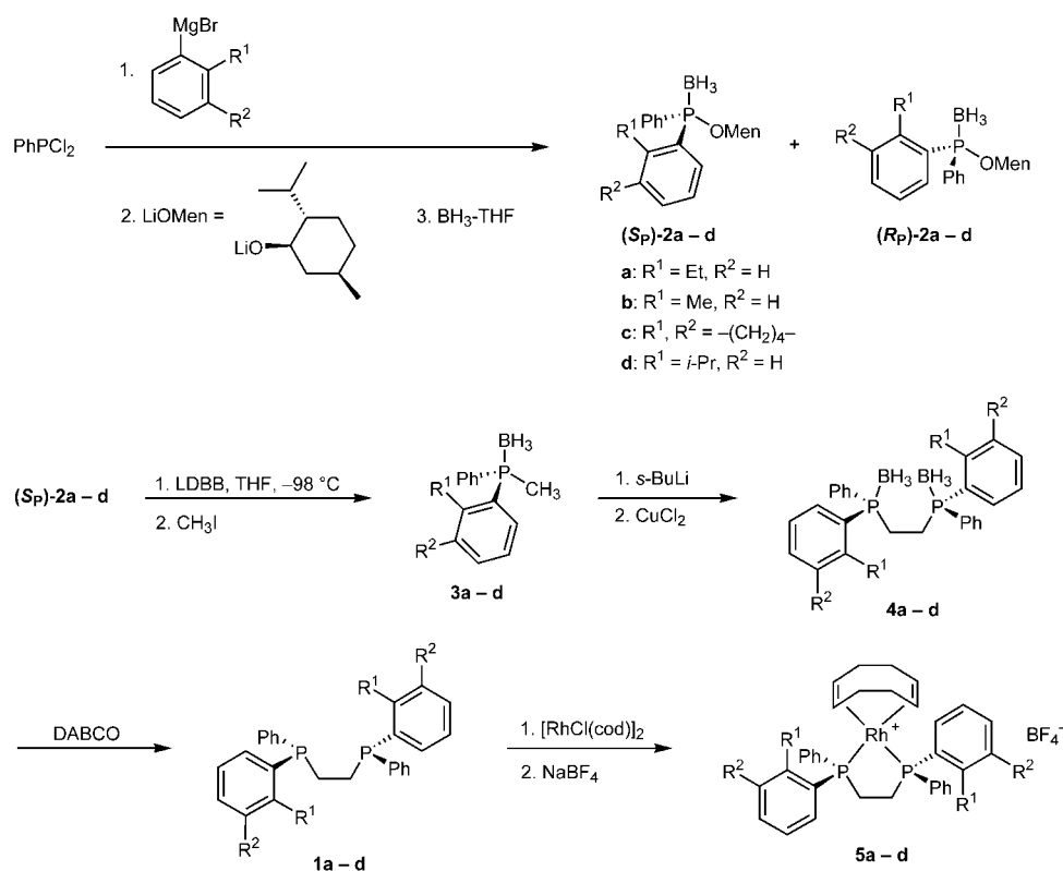
Scheme 2. Synthesis of optically active 1,2-bis[( o -alkylphenyl)phenylphosphino]ethanes and their rhodium complexes.
