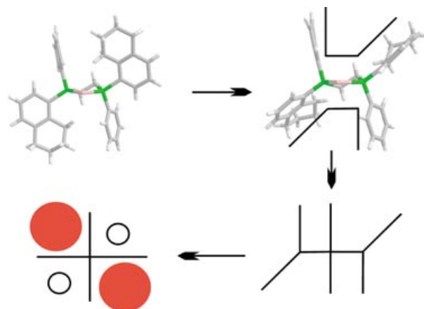
Figure 4. Schematic illustration of the possibility to regard unsubstituted phenyls of 5c as “bulky” substituents. The X-ray-based structure of 5c shown in the upper left corner is conformationally modified by rotation around two P–C bonds producing “pockets” appropriate for the coordination of a substrate in the upper right and lower left quadrants.
